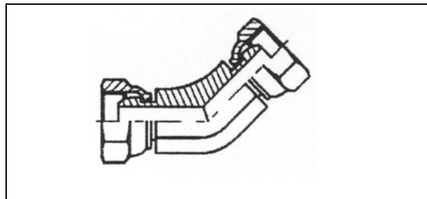
A20BF45-20BF 1"1/4-11 1"1/4-11
